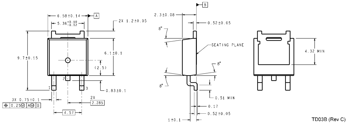
TO-252 Order Number LM78M05CDT NS Package Number TD03B
