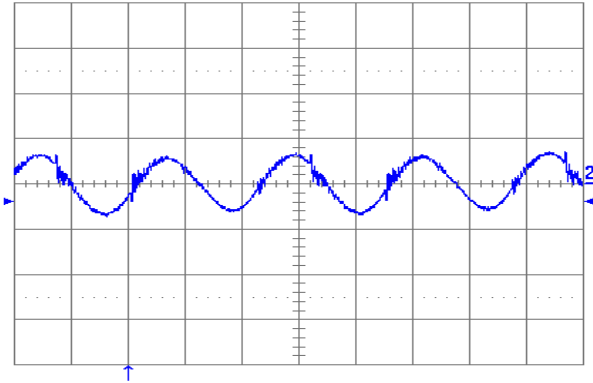
Figure 12: Input reflected-ripple current, i_s (10 mA/div.), measured \mu\text{H} at the source at full rated load current and V_{in} = 48\text{ V} . Refer to Figure 11 or test setup. Time scale: 1 \mu\text{s}/\text{div} .
