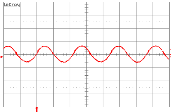
Figure 13: Input reflected ripple-current, i_c (200 mA/div.), through 10 measured at input terminals at full rated load current and V_{in} = 48\text{ V} . Refer to Figure 11 for test setup. Time scale: 1 \mu\text{s}/\text{div} .
