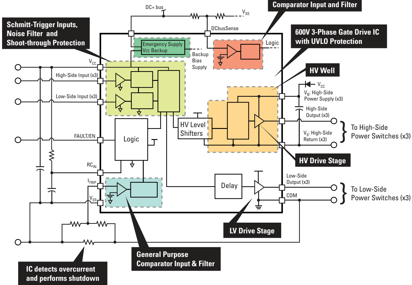
IRS26320JPbF Functional Block Diagram
