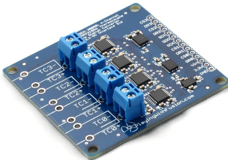
Appendix 2d: SEN-30008, Screw Terminal
