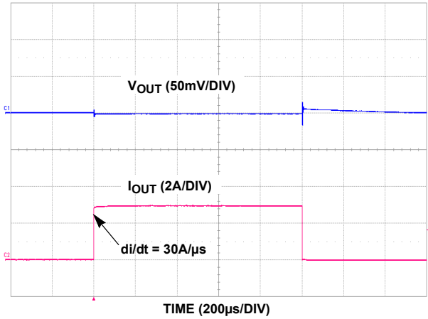
FIGURE 29. LOAD TRANSIENT 0A TO 3A, C_{OUT} = 10\mu F CERAMIC + 100 \mu F OSCON
