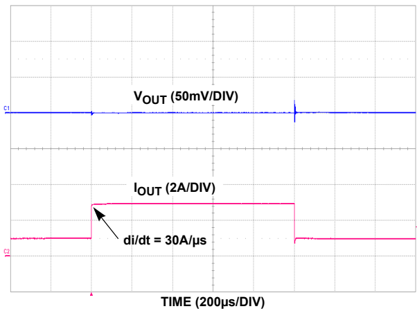
FIGURE 31. LOAD TRANSIENT 1A TO 3A, C_{OUT} = 10\mu F CERAMIC + 100 \mu F OSCON
