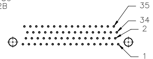
SUGGESTED HOLE PATTERN PIN OUT
