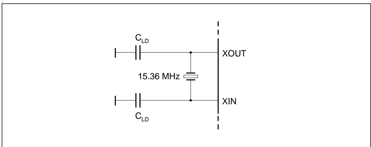
Figure 71 Crystal Oscillator
