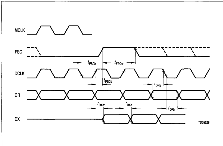
Figure 35 SDI-Switching Timing Diagram
