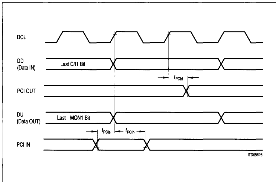
Figure 33 IOM ® -2 Bus Timing Diagram (TE-Mode)
