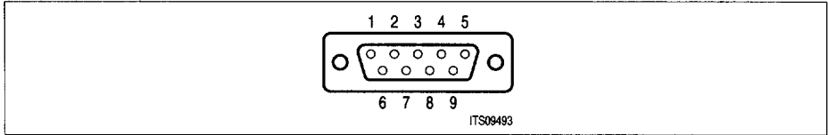
Figure 45 IOM® Connector
