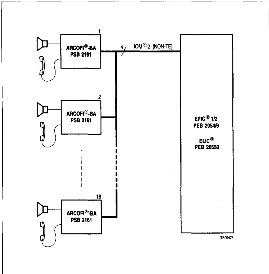
Figure 12 ARCOFI ® Line Card Application
