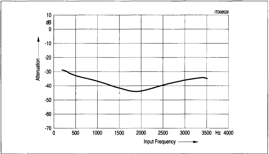
Figure 82 Transhybrid Loss
