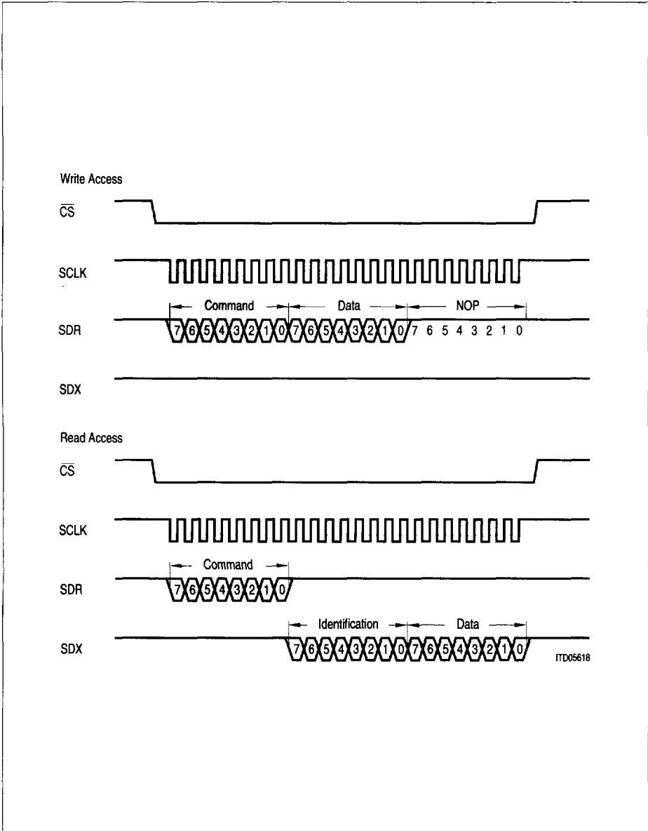
Figure 25 Serial Control Interface Timing
