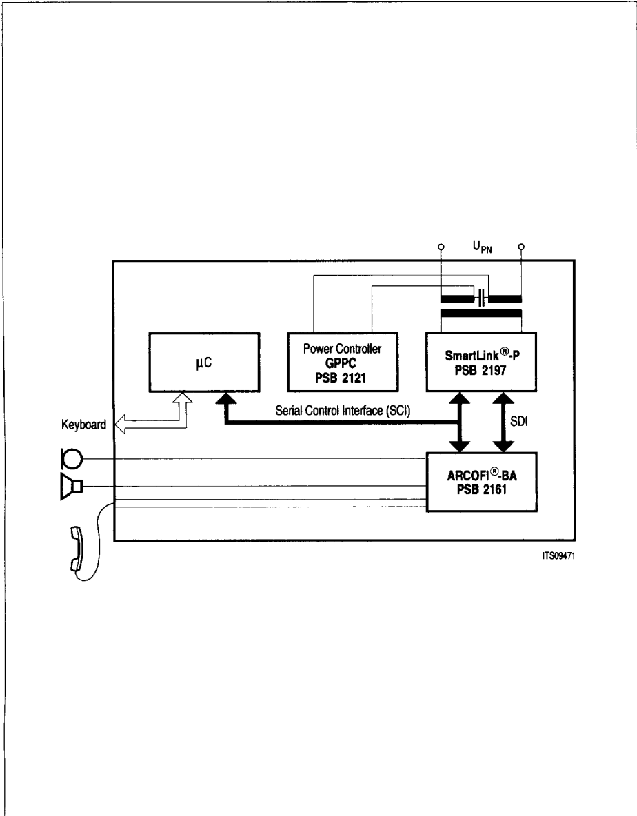
Figure 8 PABX Voice Terminal in NON-IOM ® -2 Architecture
