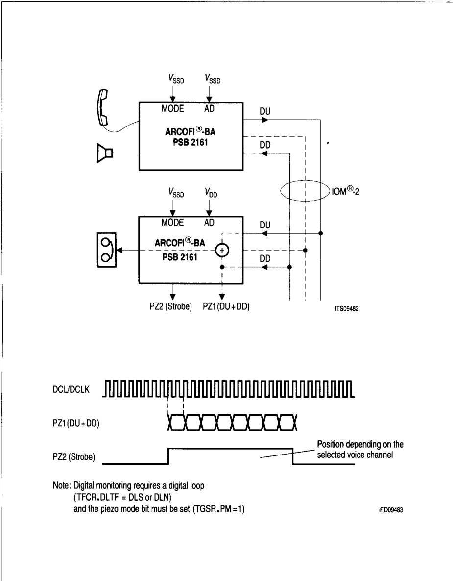
Figure 30 Configuration of the IOM®-2 TE Monitoring Mode
