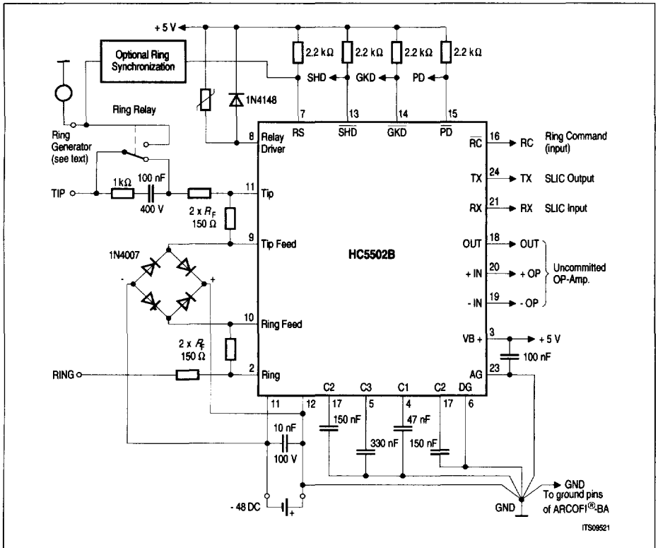
Figure 75 Circuitry for the HC5502B
