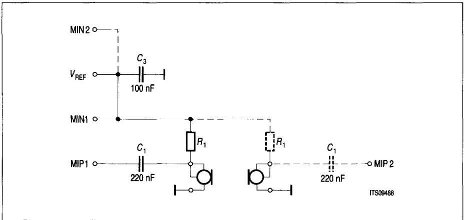
Figure 40 Interfacing Electret Microphones with Bias from V REF
