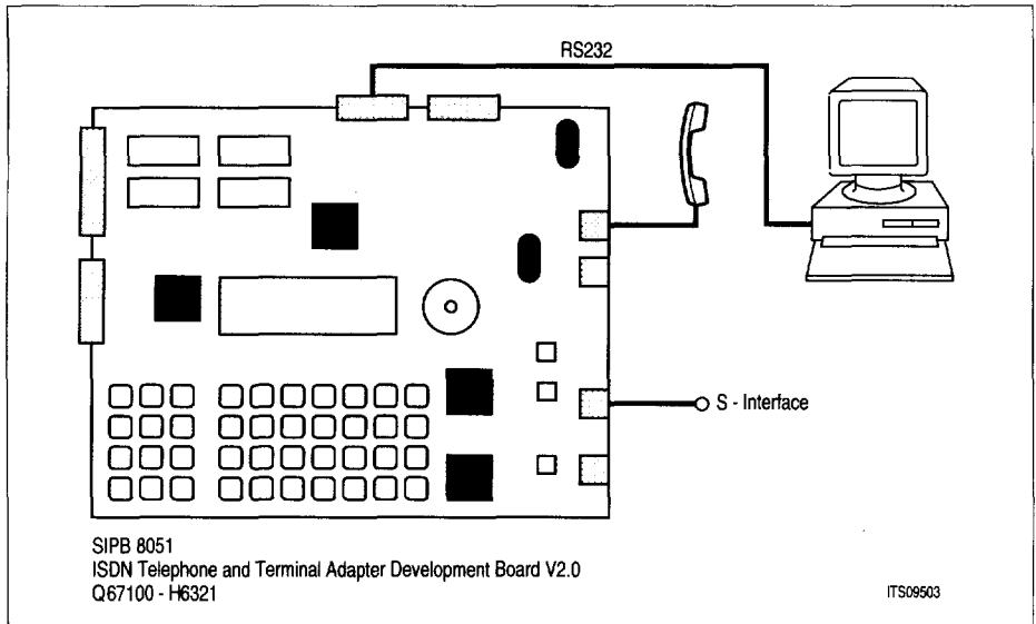
Figure 59 Setup for the SIPB 8051 Telephone Board
