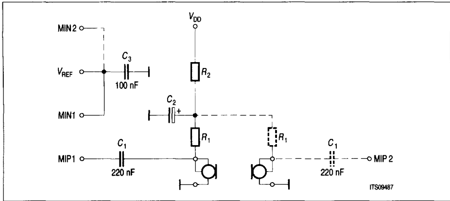
Figure 39 Interfacing Electret Microphones with Bias from V_{DD}
