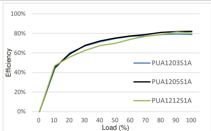
PUA12-1A Efficiency vs. load current at T_{P1} = +25^{\circ}\text{C} .
