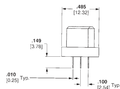
Solder Posts
