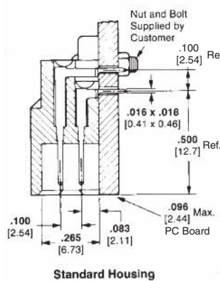
Standard Housing
