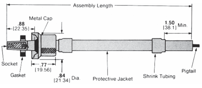
Part Number 861811
