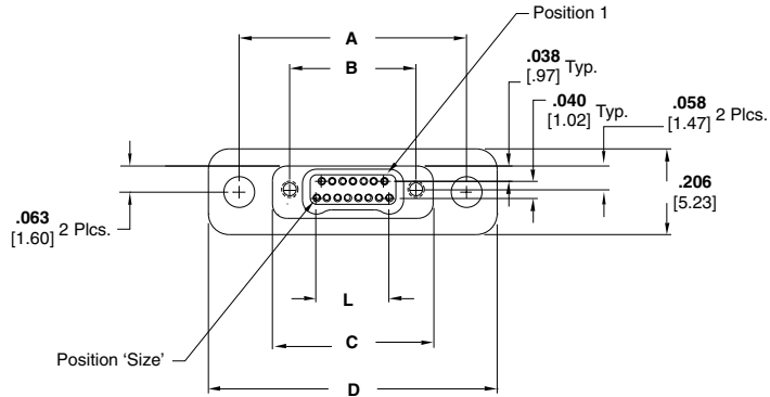
Receptacle Assembly Drawing Number 1589050
