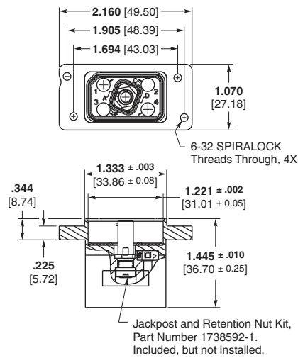
Panel Mount Receptacle (Part No. 1738950)
