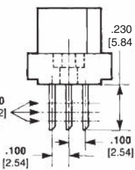
Solder Eyelet Contact
