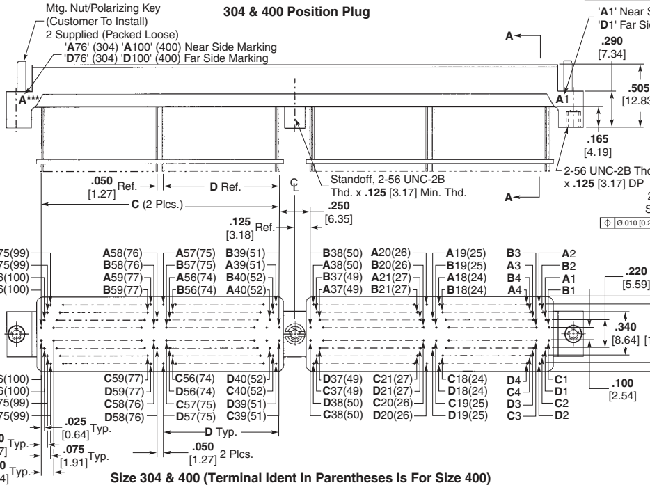
304 & 400 Position Plug
