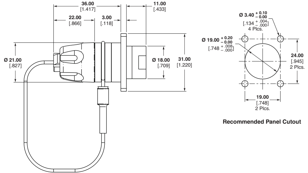
PRO BEAM Mini Low Profile, Alternate Square Flange Mount Bulkhead Connector
