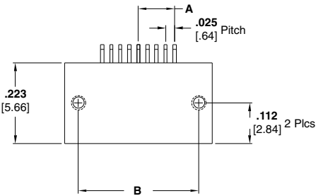
Plug Assembly Drawing Number 1589460
