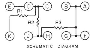
SCHEMATIC DIAGRAM
