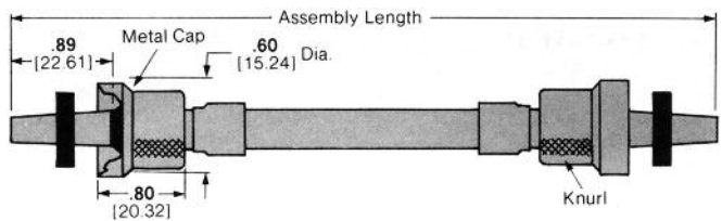
Part Number 861810
