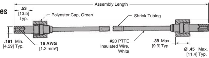
Part Number 860529
