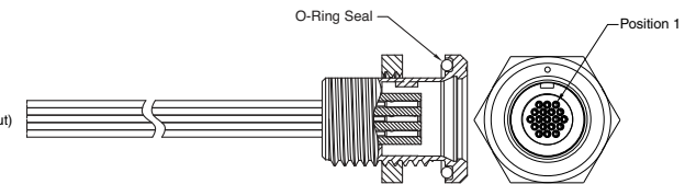
19 Position Drawing Number 1589058
