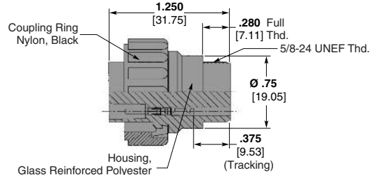
Part Number 867534-1
