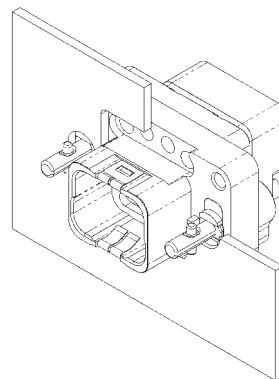
GPR1ZM05N Panel Rear Mounted Connector
