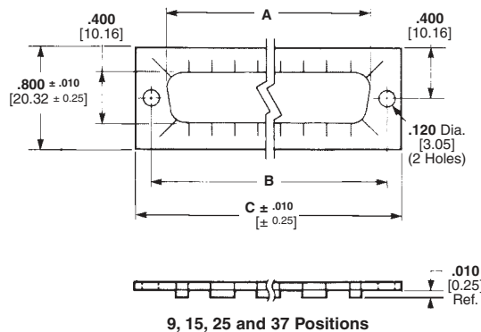
9, 15, 25 and 37 Positions
