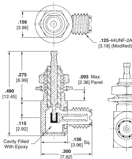
Right-Angle Receptacle 1 Part Number 141-0020-0001
