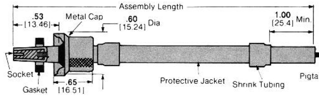
Part Number 861807
