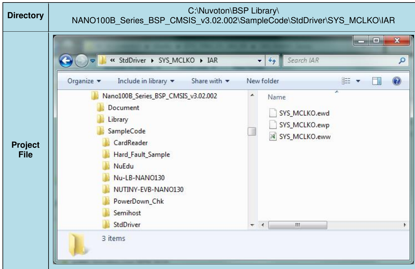
Figure 4-2 Example Directory
