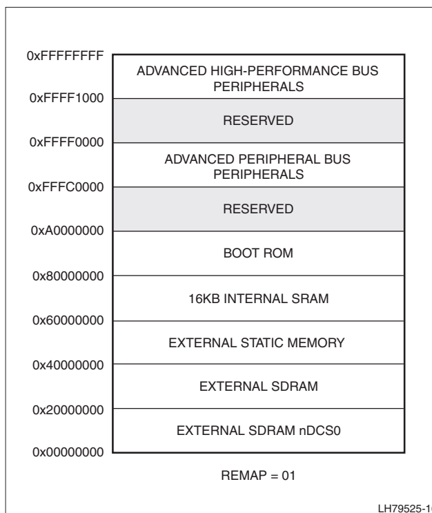
Figure 4. Memory Remap '01'
