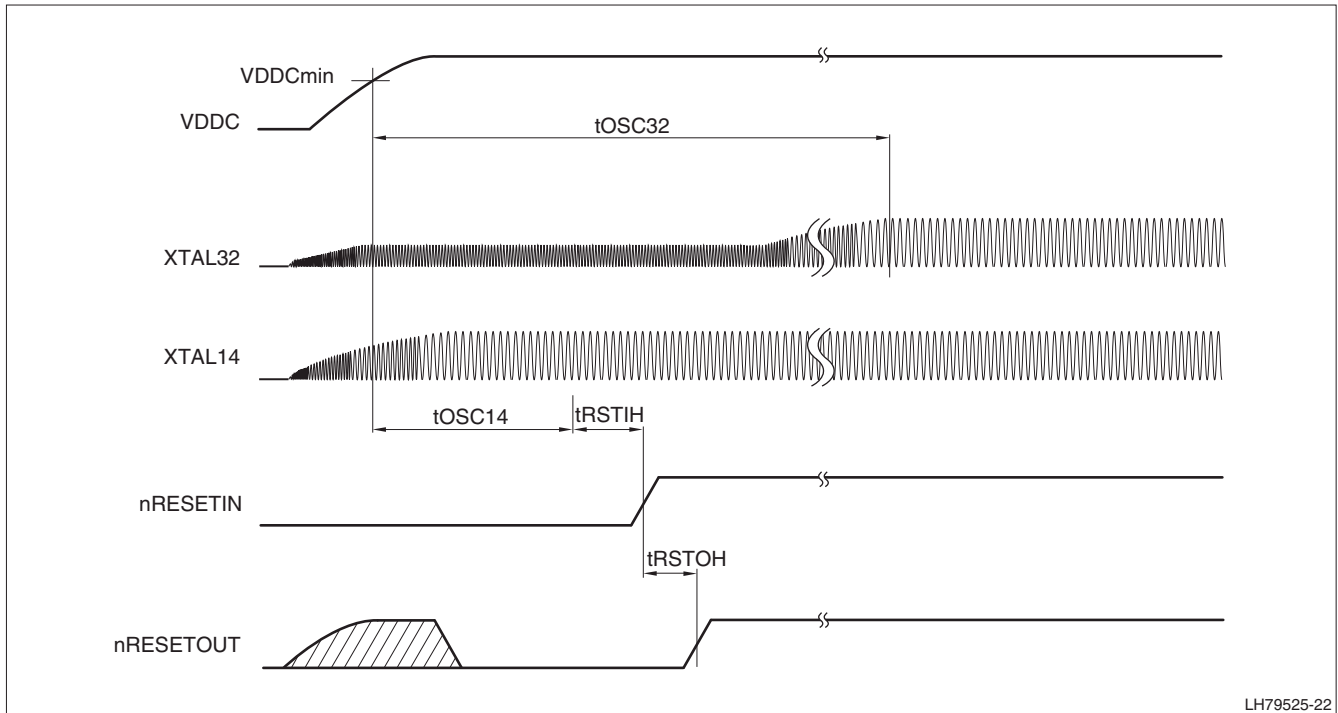
Figure 35. PLL Start-up
