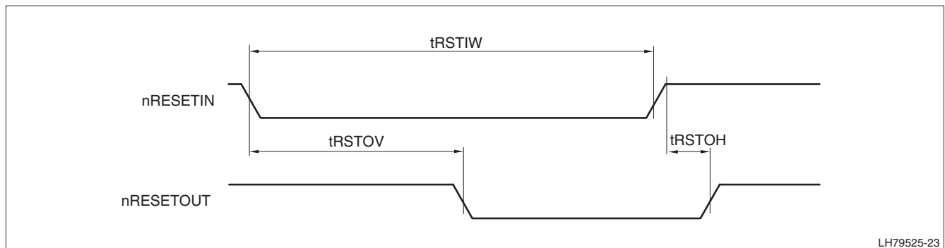
Figure 36. External Reset
