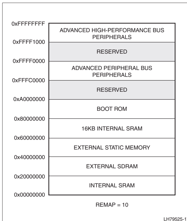
Figure 5. Memory Remap '10'
