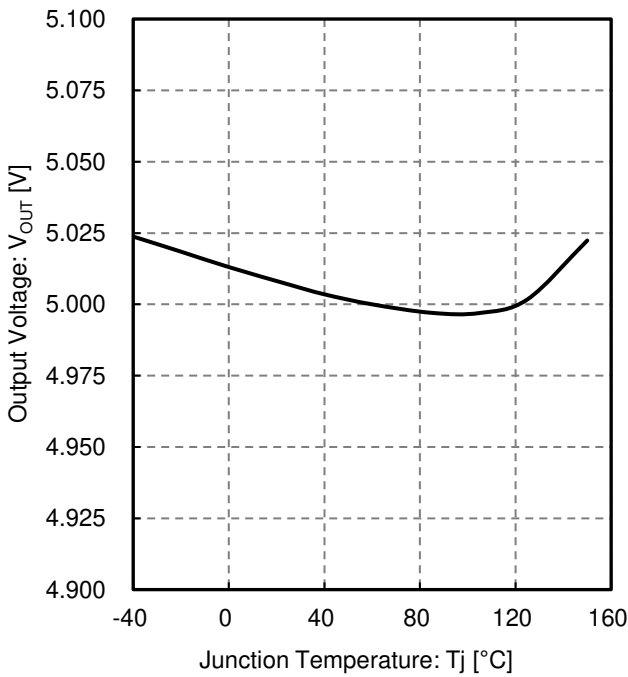
Figure 3. Output Voltage vs Junction Temperature ( I_{OUT} = 0.5\text{ mA} )
