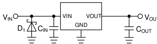
Figure 30. Surges Lower than -0.3\text{ V} is Applied to the Input
