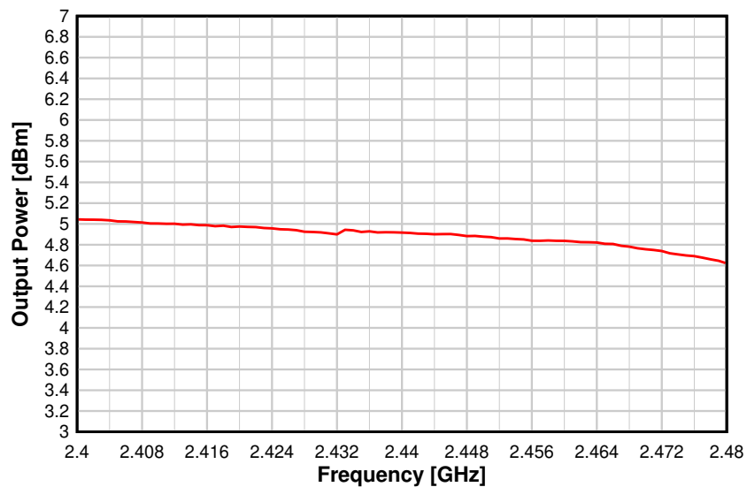
Figure 8-23. Output Power vs. Frequency (BLE 1 Mbps, 2.44 GHz, +5 dBm)
