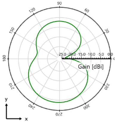
Measured at 433 MHz
