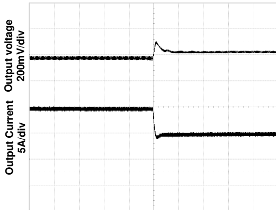
Figure 2. Transient Load Response Input voltage 12V, Output voltage 6V, Output current 10A->5A, Slew rate 2.5A/μs
