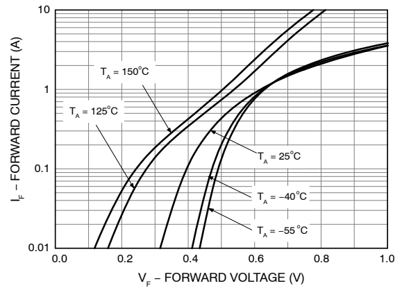
Figure 4. Typical Forward Characteristics - SS16HE
