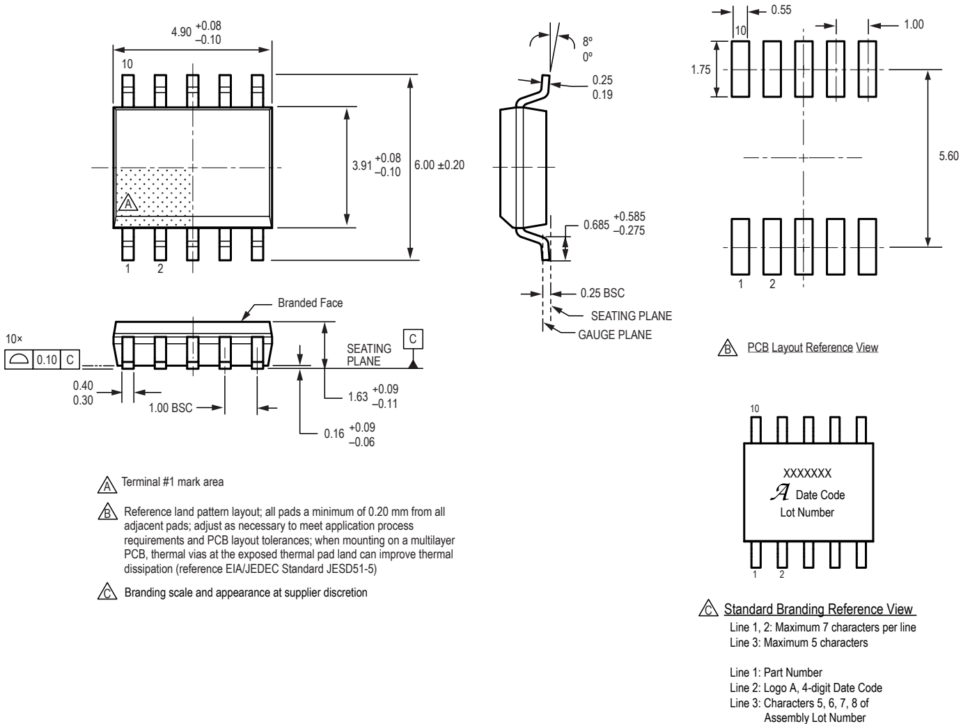
Figure 13: Package LN, 10-Pin SOIC
