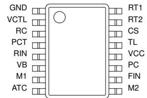
Fig.16 BA6951FS (SSOP-A16)
