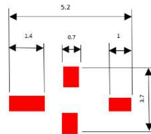
PCB Footprint
