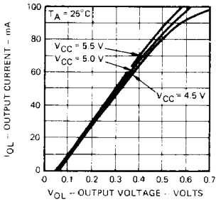
Output Low Current Versus Output Low Voltage
