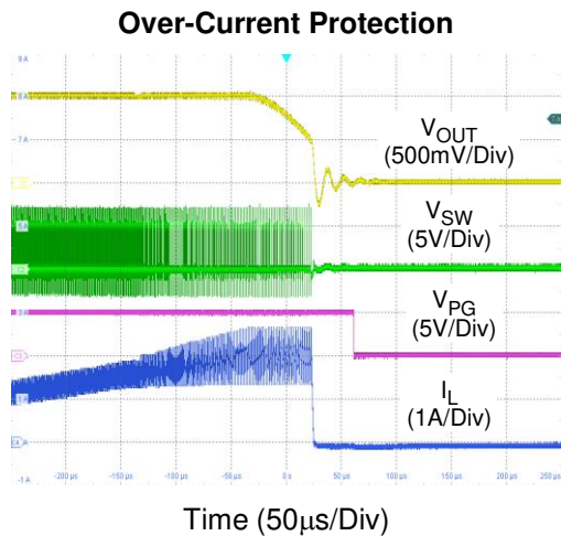
Figure 3. Over-Current Protection
