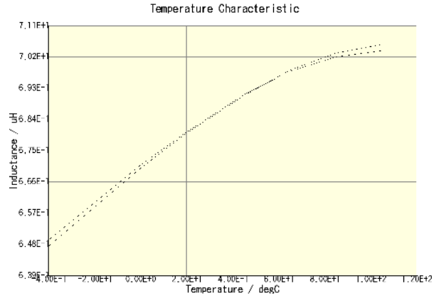
CLF12555T-680M-CA(DC = 0A)
