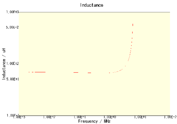
CLF12555T-680M-CA
