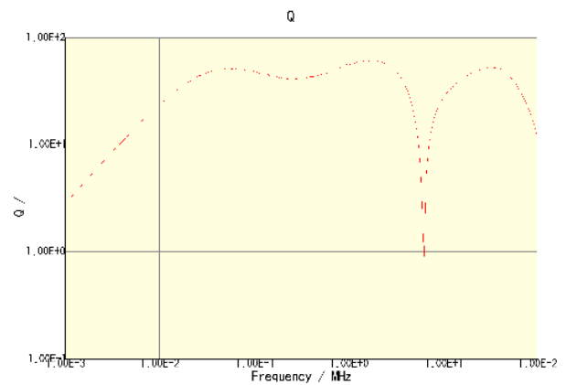
CLF12555T-680M-CA
