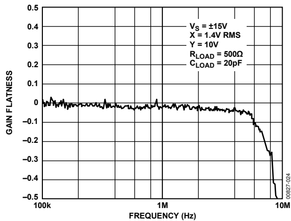
Figure 6. Gain Flatness, 300 kHz to 10 MHz, R_{LOAD} = 500\text{ }\Omega
