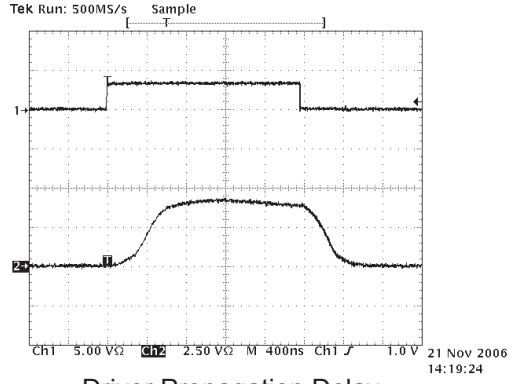
Driver Propagation Delay (SP3083E-SP3085E)
