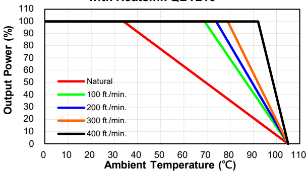
CQB150W Derating Curve with Heatsink QBT210
