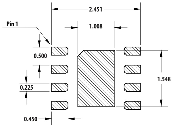
Stencil Opening
