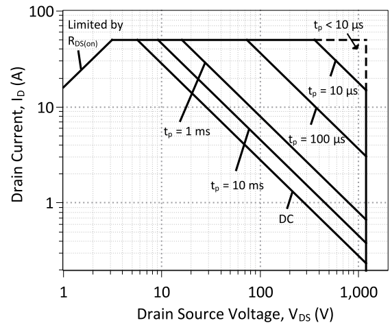
Figure 18: Forward Bias Safe Operating Area at T_C = 25\text{ °C}
