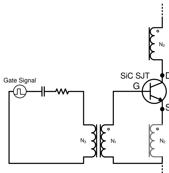
Figure 28: Simplified Current Controlled Proportional Driver
