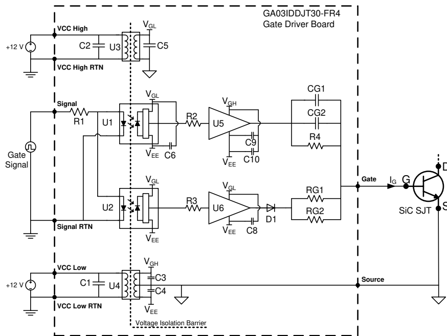
Figure 23: Topology of the GA03IDDJT30-FR4 Two Voltage Source gate driver.
