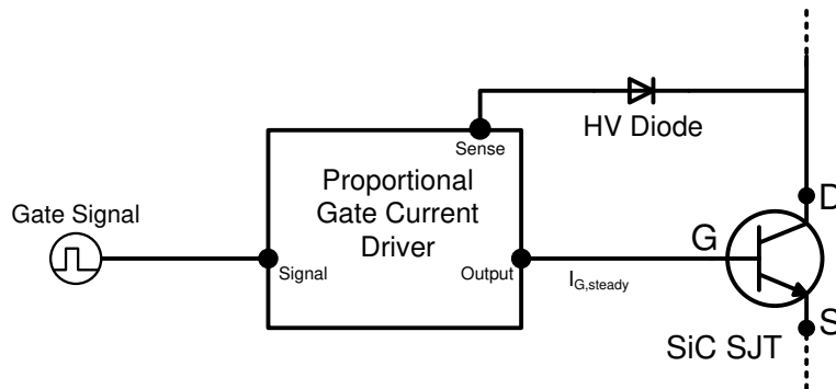
Figure 27: Simplified Voltage Controlled Proportional Driver
