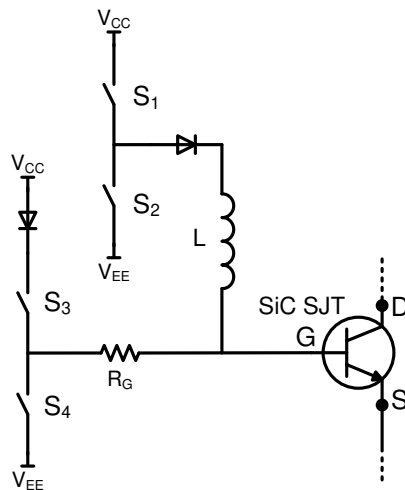
Figure 26: Simplified Inductive Pulsed Drive Topology
