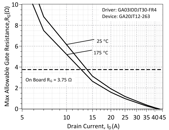
Figure 25: Maximum gate resistance for safe operation of the GA20JT12-247 at different drain currents using the GA03IDDJT30-FR4 board.
