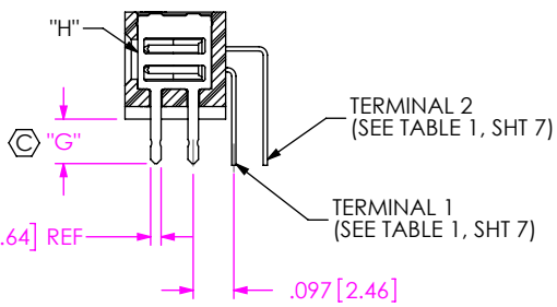
SECTION "J"-"J"
