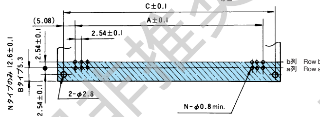
推奨取付寸法 Recommended mounting dimensions
