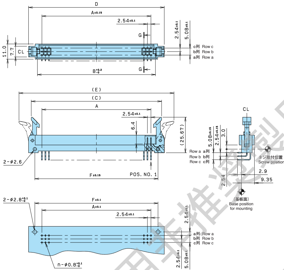
推奨取付寸法 Recommended mounting dimensions
