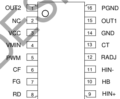
SSOP-16
