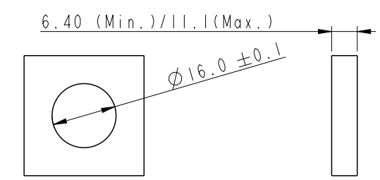
Panel cut out (hole type)
