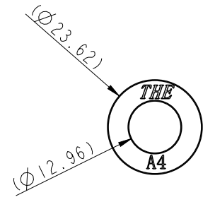
Washer
