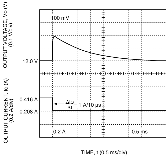
Figure 5. CW025 Dual Output-Series Typical 12 V Output Voltage Response to a Step Load Change from 50% to 25% of I_{o,max} at V_i = V_{i,nom} and T_c = 25\text{ }^\circ\text{C}
