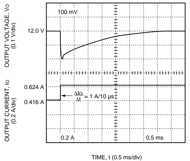
Figure 8. CW025 Dual Output-Series Typical 12 V Output Voltage Response to a Step Load Change from 50% to 75% of I_{o,max} at V_i = V_{i,nom} and T_c = 25\text{ }^\circ\text{C}
