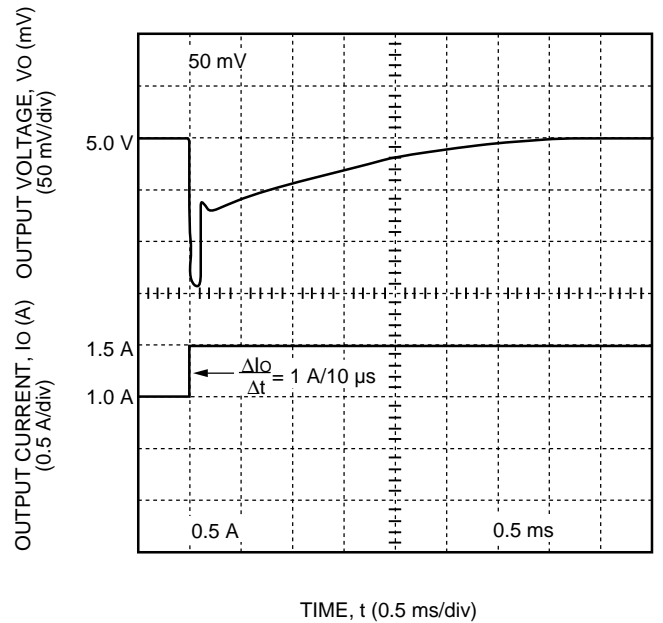
Figure 7. CW025 Dual Output-Series Typical 5 V Output Voltage Response to a Step Load Change from 50% to 75% of I_{o,max} at V_i = V_{i,nom} and T_c = 25\text{ }^\circ\text{C}
