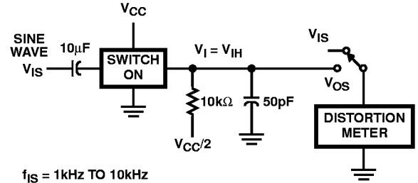
FIGURE 6. TOTAL HARMONIC DISTORTION TEST CIRCUIT
