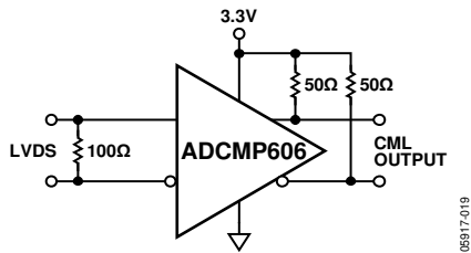
Figure 20. LVDS to CML on the ADCMP606
