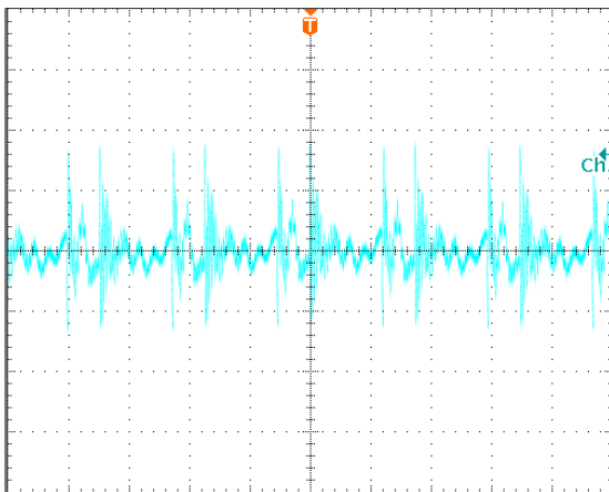
Output voltage ripple at nominal input voltage and max load current (20mV/div, 2µs/div) Load cap: 10µF, tantalum capacitor and 1µF ceramic capacitor. Bandwidth: 20MHz.
