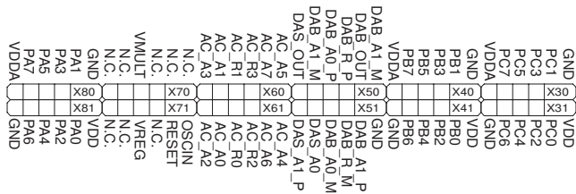
Figure 3 : XE8000EV104 connectors
