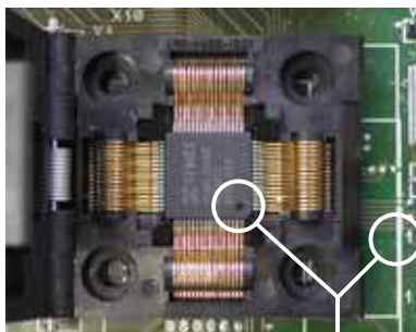
pin 1 marker
