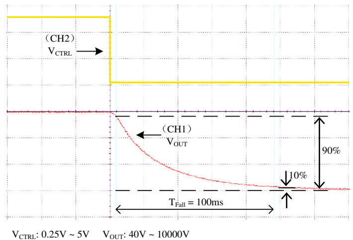
Figure 7. Fall Time
