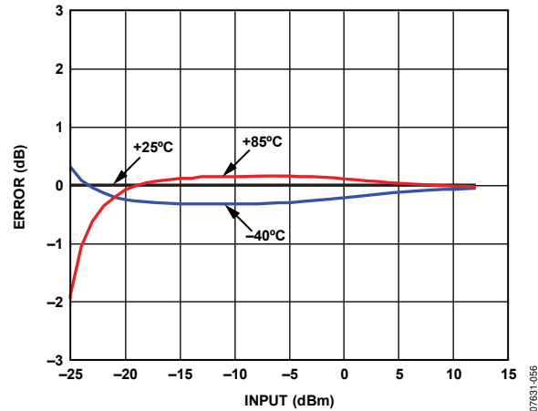
Figure 56. VRMS Error from +25°C Output Voltage at -40°C, +25°C, and +85°C After Ambient Normalization, Frequency 1900 MHz, Supply 3.0 V
