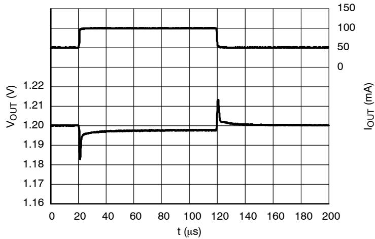
Figure 35. Load Transients, 1.2 V Version, I_{OUT} = 50 - 100 mA, t_R = t_F = 0.5 \mu s, V_{IN} = 2.2 V
