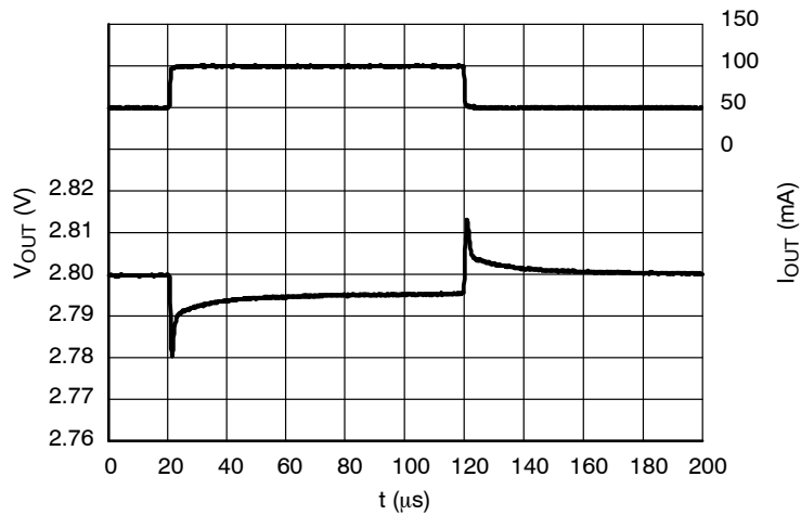
Figure 36. Load Transients, 2.8 V Version, I_{OUT} = 50 - 100 mA, t_R = t_F = 0.5 \mu s, V_{IN} = 3.8 V
