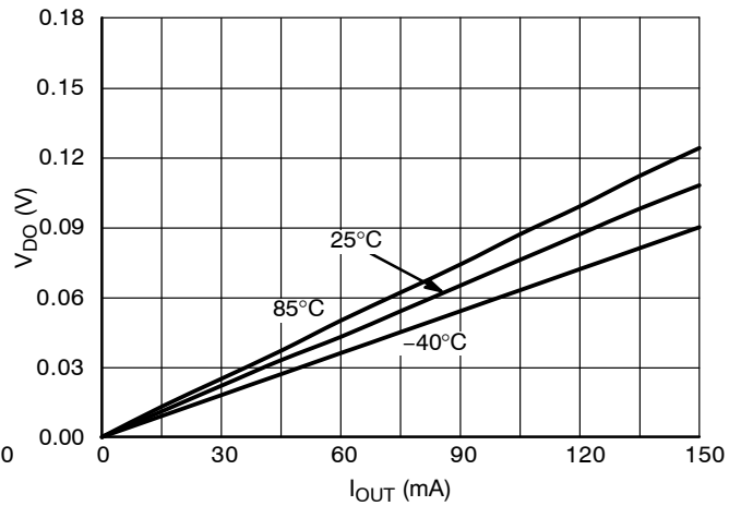
Figure 6. Dropout Voltage vs. Output Current 2.8 V Version
