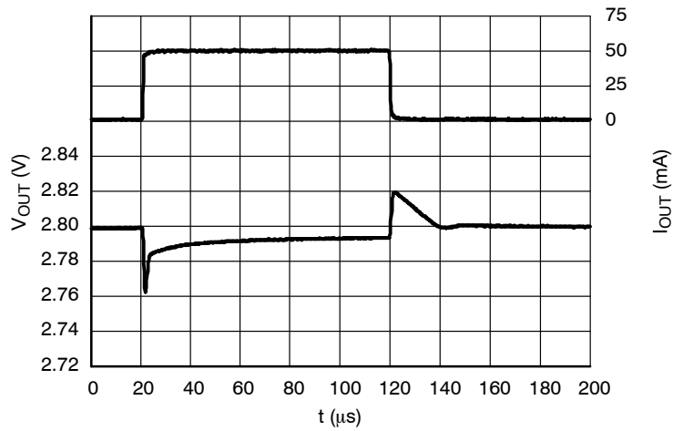
Figure 34. Load Transients, 2.8 V Version, I_{OUT} = 1 - 50 mA, t_R = t_F = 0.5 \mu s, V_{IN} = 3.8 V, AE = V_{IN} V
