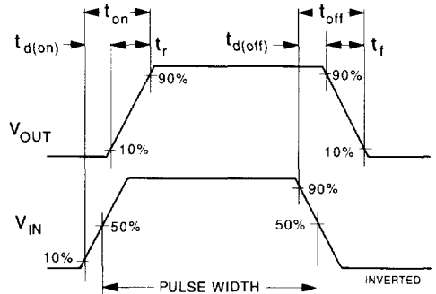
Figure 12. Switching Waveforms.
