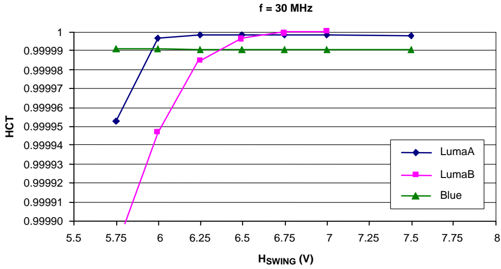
Figure 9. Typical CTE Performance vs. H Clock Levels
