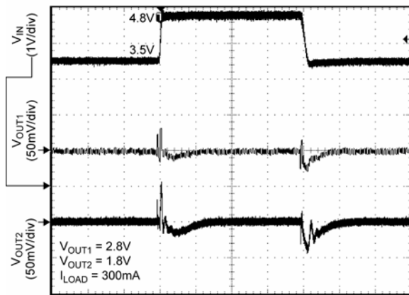
Time (10µs/div)
