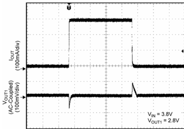
Time (40µs/div)
