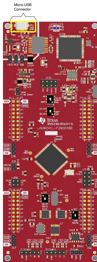
Figure 2-4. Micro-USB Connection
