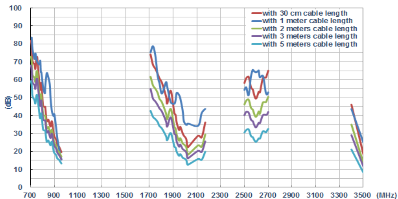
Peak Gain (ANTENNA_2 on the 2mm ABS)
