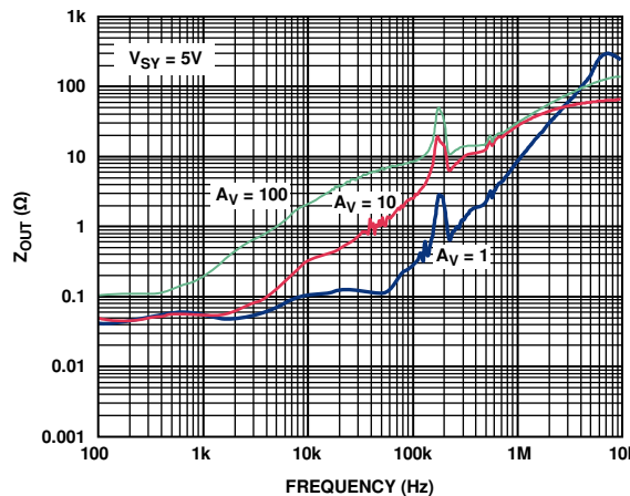
Figure 37. Closed-Loop Output Impedance vs. Frequency
