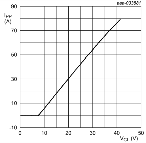
Fig. 6. Dynamic resistance with positive clamping; typical values
