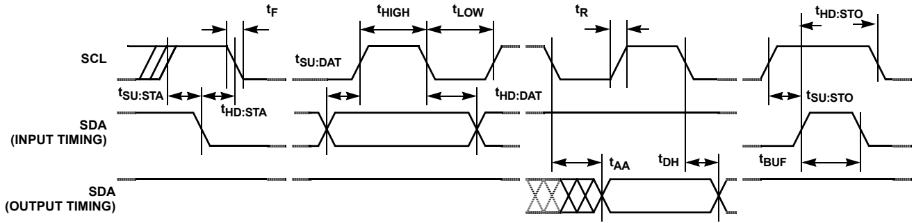
FIGURE 1. BUS TIMING
