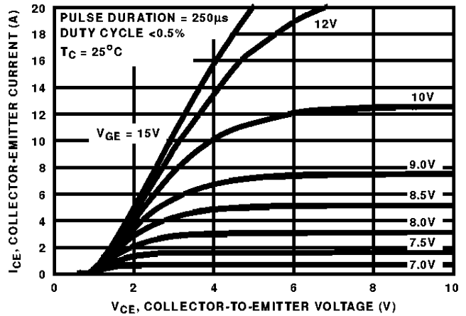
FIGURE 2. SATURATION CHARACTERISTICS
