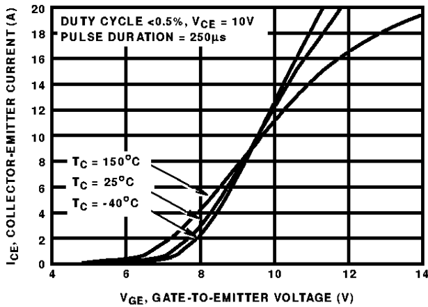
FIGURE 1. TRANSFER CHARACTERISTICS
