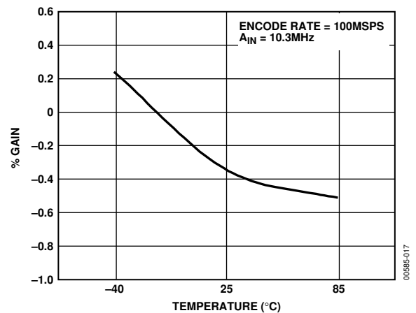
Figure 17. ADC Gain vs. Temperature (with External 1.25 V Reference)
